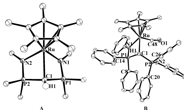
Figure 1. ORTEP drawings (50% vibrational ellipsoids). (A) (C 5 -Me 5 )Ru[HC(PPh 2 NPh) 2 ]: Ru–N1 2.229(2); Ru–N2 2.226(1); Ru–C1 2.273(2) Å; ∠N1–Ru–N2 82.68(5); ∠C1–Ru–N1 70.22(5); ∠C1–Ru–N2 71.25(5); ∠P1–C1–P2 120.87(9)°. (B) (C 5 Me 5 )Ru(CO)[η 2 -HC(PPh 2 -NPh) 2 ]: Ru–C48 1.863(2); Ru–C1 2.211(2); Ru–N1 2.156(2) Å; ∠C48–Ru–N1 93.79(10); C48–Ru–C1 97.17(10); C1–Ru–N1 72.49(7); C8–P1–C14 106.80(11); C20–P2–C26 107.31(11); C1–P1–N1 99.37(10); C1–P2–N2 109.58(11); P2–C1–P1 119.14(14)°.
